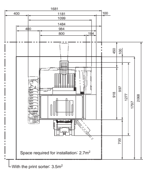
Space required for installation (Unit: mm)
