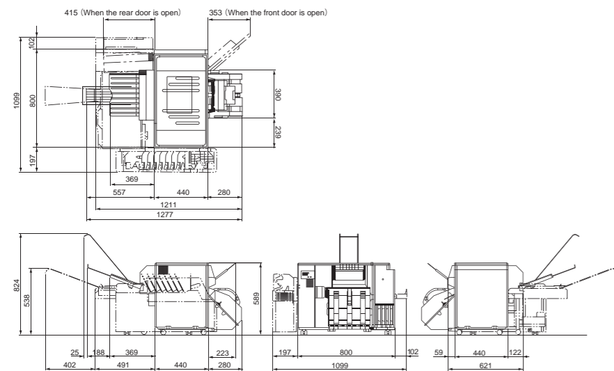
External view (Unit: mm)
